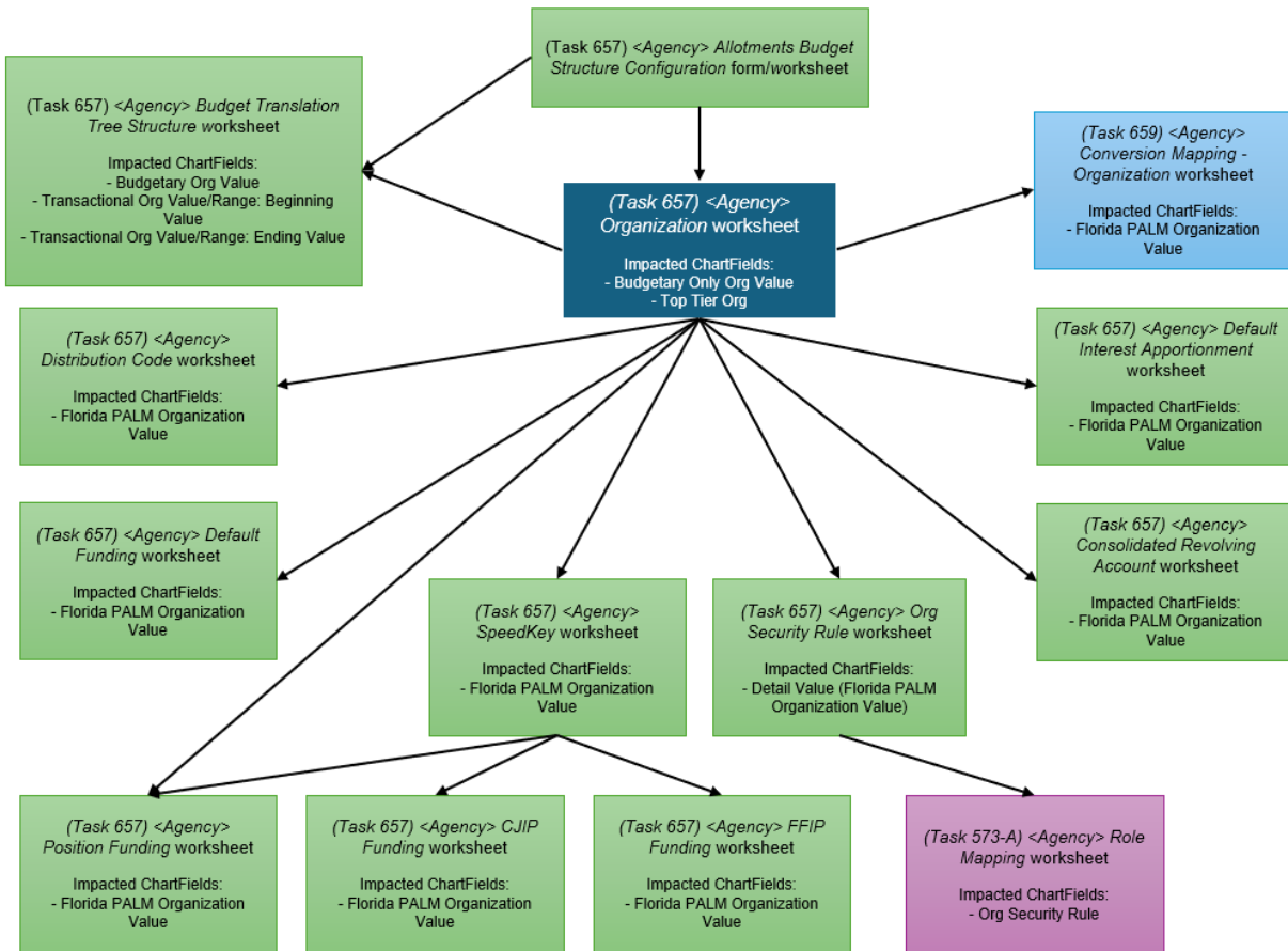
Figure 3: Cross-worksheet Connections for CRA
